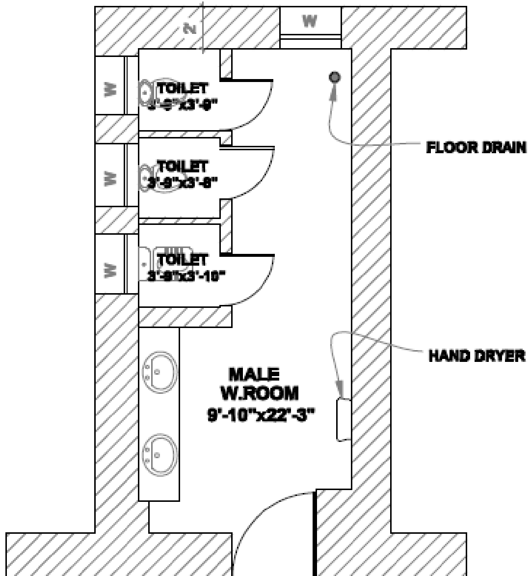
EXISTING GROUND FLOOR WASHROOM PLAN
